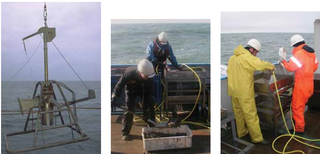
Figure 5. Reineck boxcorer for sampling infauna. Sampling size 0.07 \text{ m}^2 to a depth of 40 cm. Samples are washed over 1 mm sieves.
