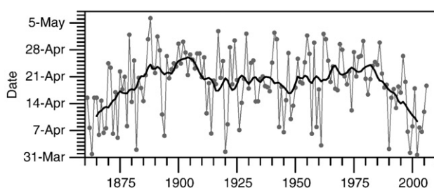
Fig. 10. Long-term time series of the trigger date for the spawning of Macoma balthica when the Marsdiep SST surpassed 8.3 °C, derived from the monthly mean SST values (thin grey line with symbols), and the low-pass version of these dates, obtained by applying a 10 year running mean (full thick black line).
