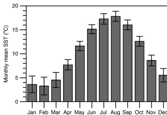
Fig. 7. Averaged monthly mean SST with standard deviation for the period 1861–2006. The error bars show the standard deviation, derived from the individual monthly averages.
