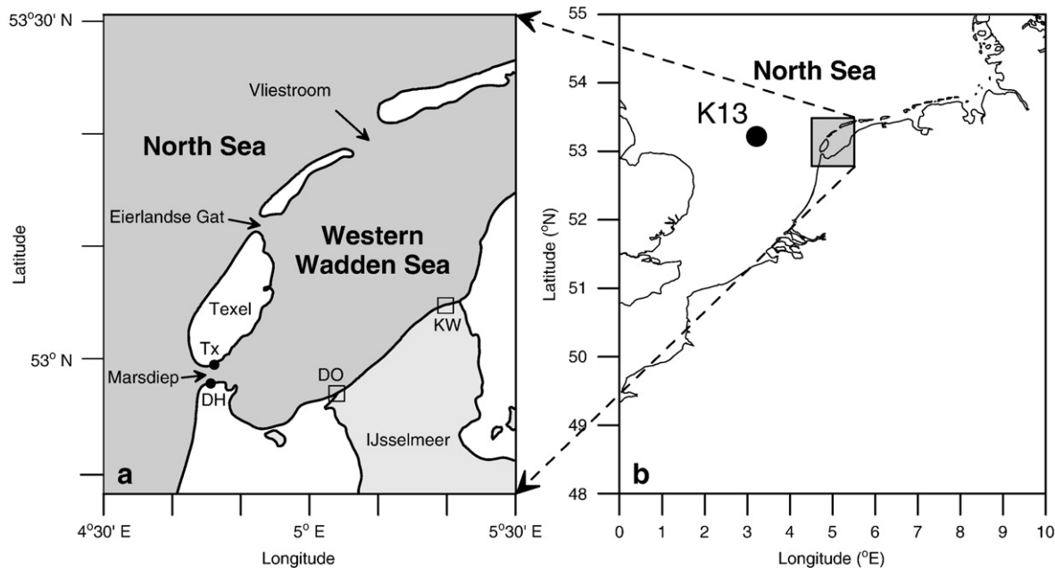
Fig. 1. Maps showing the western Wadden Sea (a) and the surrounding southern North Sea (b). The main connections of the Wadden Sea with the North Sea are the tidal inlets Marsdiep and Vliestroom. The inlet Eierlandse Gat only flushes a small sub-basin of the western Wadden Sea. Since 1932 the Wadden Sea has become separated from the former Zuiderzee, presently the freshwater lake IJsselmeer. The latter discharges surplus freshwater via outlet sluices near Den Oever (DO) and Kornwerd (KW). Since 1861 sea surface temperatures were daily measured from the sea dyke in Den Helder (DH), while since 1947 similar measurements were measured from the sea dyke of the Wadden Island Texel. The black symbol in (b) shows the position of the K13 oil platform.
