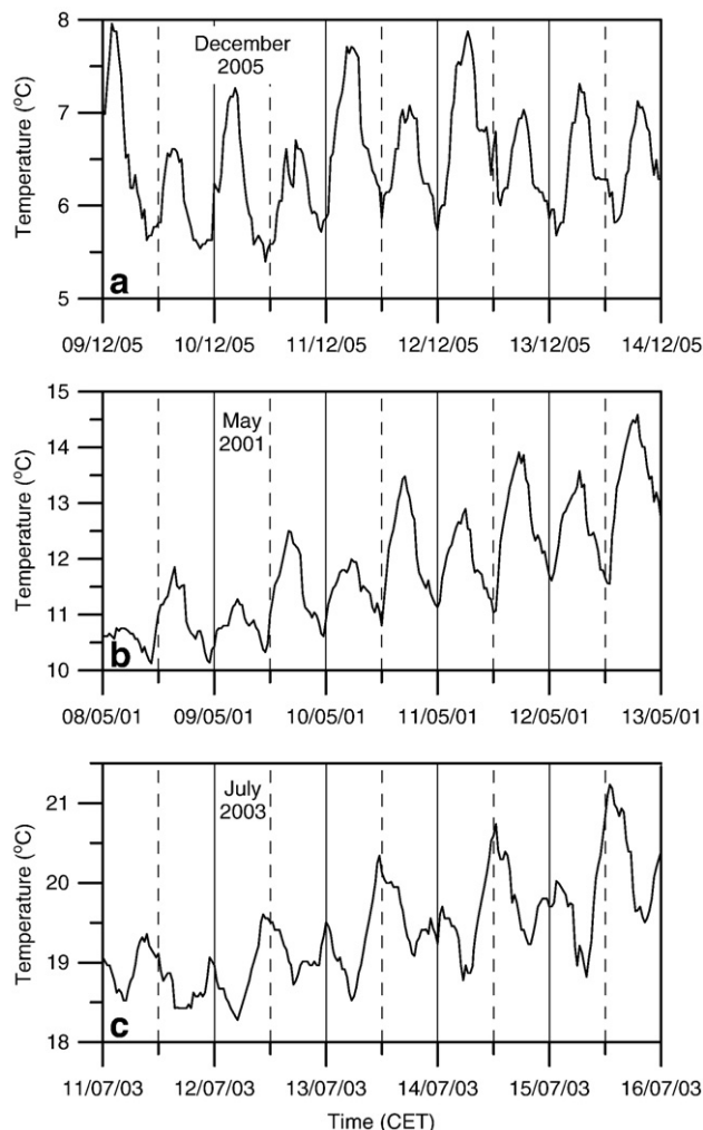
Fig. 4. Exemplary plots of the sea surface temperature in the Marsdiep, showing the daily inequality for December 2005 (a), May 2001 (b) and July 2003 (c). The vertical full lines indicate Midnight, Central European Time, the dashed line indicate noon. The time labels follow the European date/month/year convention.
