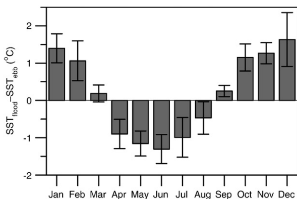
Fig. 3. Monthly mean sea surface temperature differences between flood and ebb, based on 5 years continuous observations from 2002 until 2006. The error bars show the standard deviations, derived from the single month averages of the difference.
