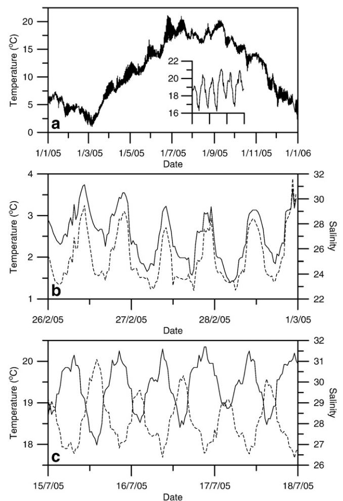
Fig. 2. A plot of the sea surface temperature in the Marsdiep recorded every 30 min throughout 2005 (a), a plot of temperature and salinity during 3 days in the winter of 2005 (b), and a similar plot for the summer of 2005 (c). The date labels follow the European date/month/year convention. The temperature records are shown as a full line, while the salinity is presented by the dashed line. The inset in (a) shows the large temperature variability from 23 to 25 June 2005.
