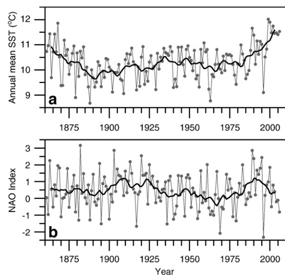
Fig. 9. Long-term time series of (a) the annually average SST and (b) the winter NAO index (December to March). The thin grey lines with symbols represent the annual data, the thick full black lines the 10 year running mean.
