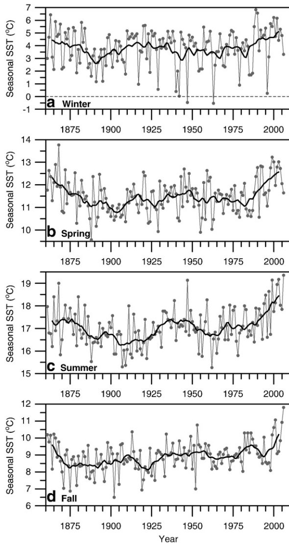
Fig. 8. Long-term time series of seasonally averaged SST (thin grey line with symbols) for the (a) Winter (January to March), (b) Spring (April to June), (c) Summer (July to September), and (d) Fall (October to December). The thick black line represents the 10 year running mean.
