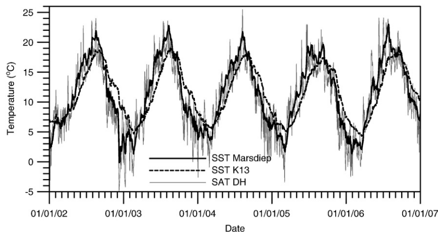
Fig. 6. Five years of daily mean sea surface temperature data from the Marsdiep (thick full line) platform K13 ( 53^{\circ}13'\text{N} , 3^{\circ}13'\text{E} , 27 m depth) in the North Sea (thick dashed line), and the daily mean surface air temperature from the meteorological station at the airport De Kooij near Den Helder (thin grey full line). The data labels follow the European date/month/year convention.
