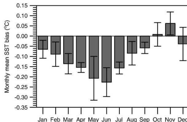
Fig. 5. Plot of the monthly SST bias ( T_{8AM} - T_{cont} ), constructed from monthly mean SSTs derived from 08:00 AM SST values, and from the continuous observations during the 5 years from 2002 until 2006. The error bars show the standard deviations, derived from the individual monthly mean SST values.
