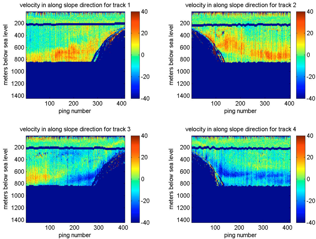
Fig. 7 Raw along slope data of first four tracks with towed body at 200 m (Erik van Sebille/Selma Huisman).
