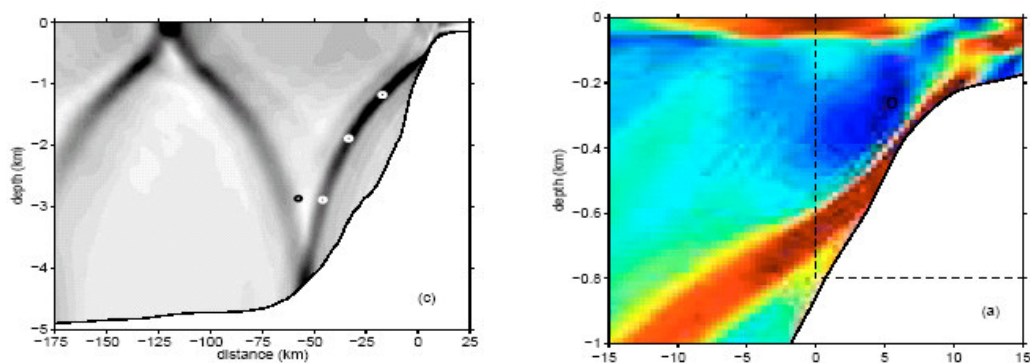
Fig. 1. Numerical model (T. Gerkema) of internal tidal beams in the Bay of Biscay: left overview; right detail.
