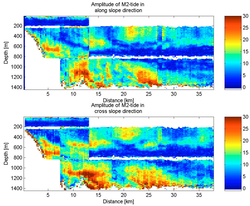
Fig. 8 Preliminary analysis of tidal amplitude in cm/s, with down- and upward sloping high amplitude bands (Erik van Sebille/ Selma Huisman).
